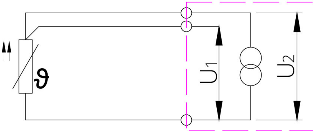
Dreileiter three-wire
